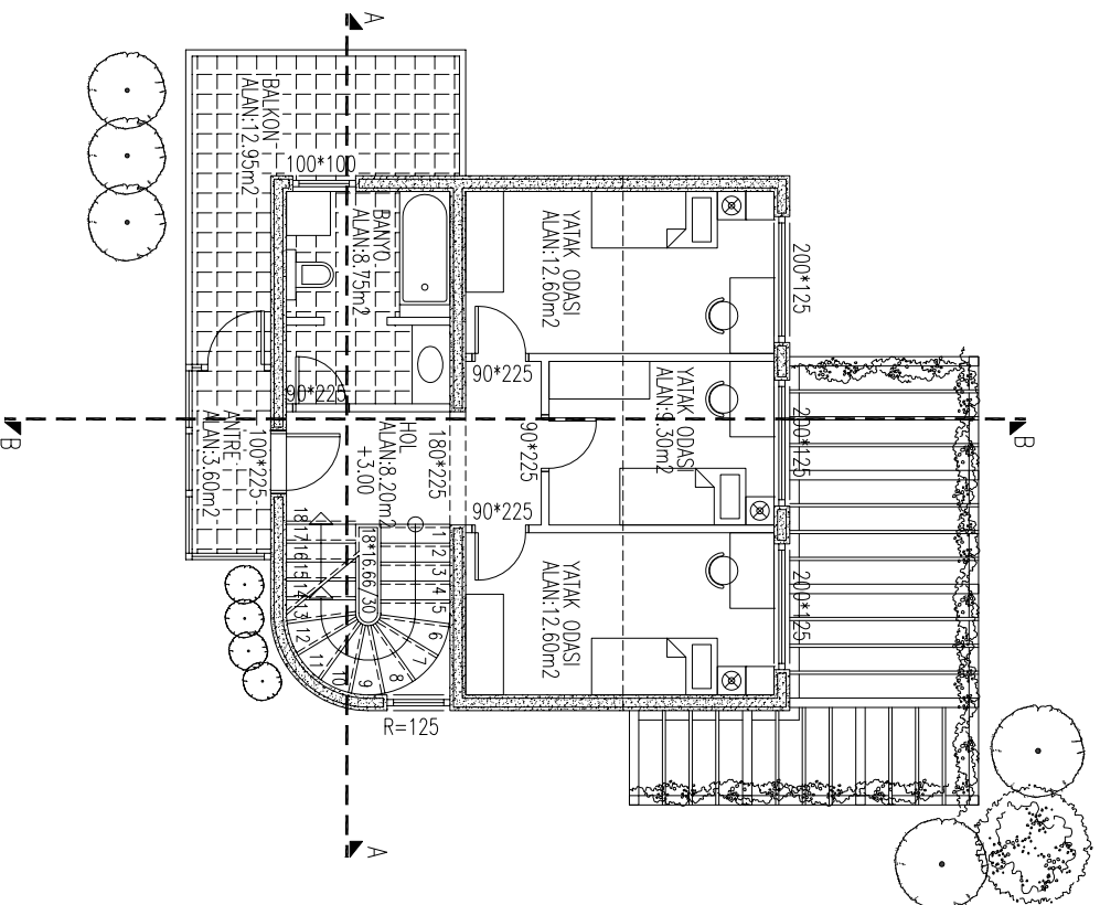
1.KAT PLANI 86.75m 2
