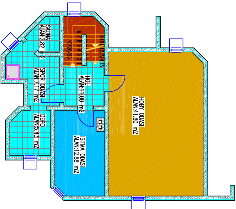
BODRUM KAT PLANI
