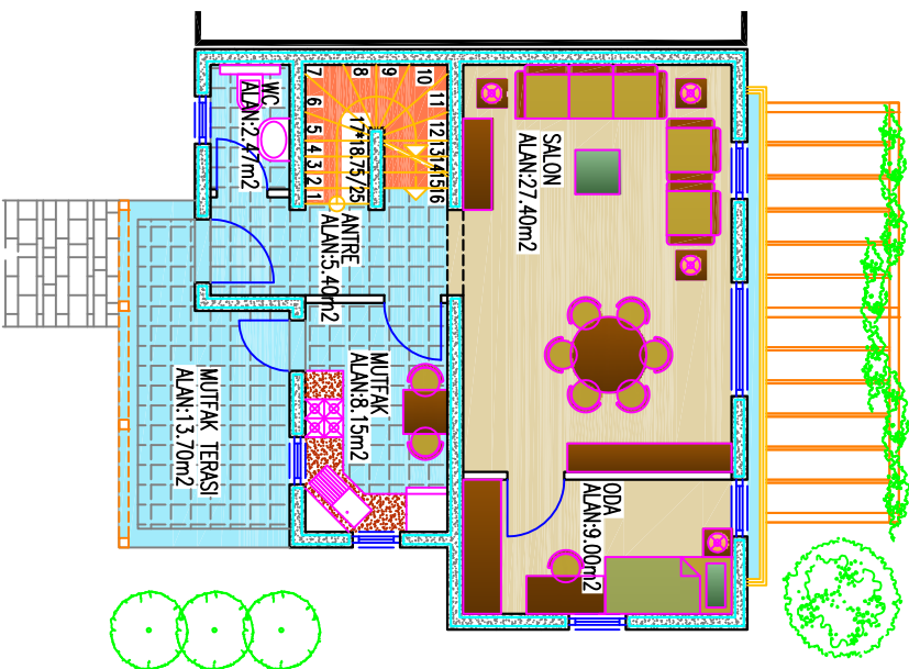
ZEMİN KAT PLANI 71.20 M 2
